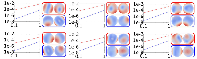
Linear and quadratic errors. Sphere radius : 1
